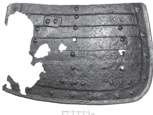
Picture 5. Pikeman's tasset (Photo by V. Abramauskas)
