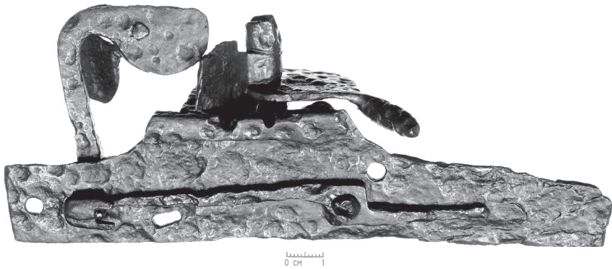
Picture 1. Matchlock mechanism (Photo by V. Abramauskas)
