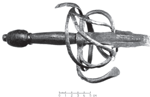
Picture 3. Swept hilt rapier (Photo by V. Abramauskas)
