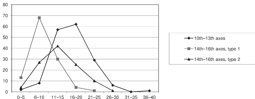
Figure 5. Blade angle relative to the shaft. Comparative diagram
